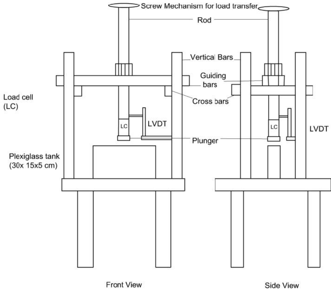
Figure: Basic model of Optical Loading Frame
